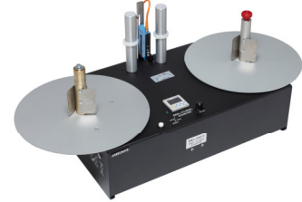
RRC-330-US Ultrasonic Reel-to-Reel Counter uses an ultrasonic detector to count almost any type of label, including transparent, semi-transparent and opaque labels. HWD: 14.5" x 32.5" x 13" (368-mm x 826-mm x 330-mm)
