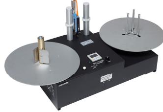
RRC-330-UA with 3" Unwind and Adjustable 1"- 4" Rewind Shaft. HWD: 13" x 32.5" x 13" (330-mm x 826-mm x 330-mm)
